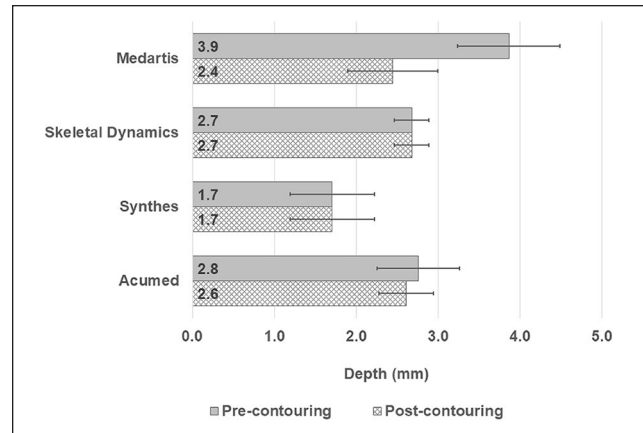
Figure 6. Bone to plate surface depth (distal) pre- and postcontouring means and standard deviations.
